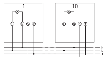
theLeda P12, theLeda P24 (Connection Master / Master)
