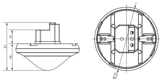
Ceiling installation box 73A Details page 337
