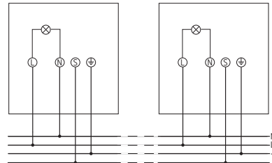
theLeda P12, theLeda P24L (Connection Master / Slave)
