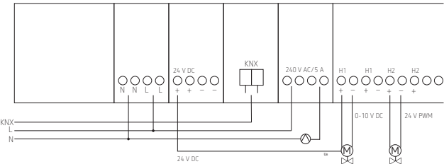
HMT 6 S KNX
